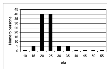
Istogramma equi-width
